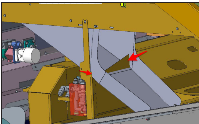
Interference of right side trash chute with existing shielding.
