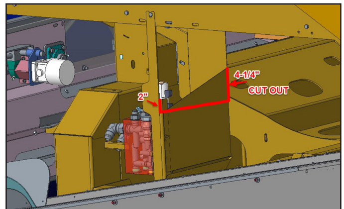
The shielding must be modified for the right side chute to be installed.
